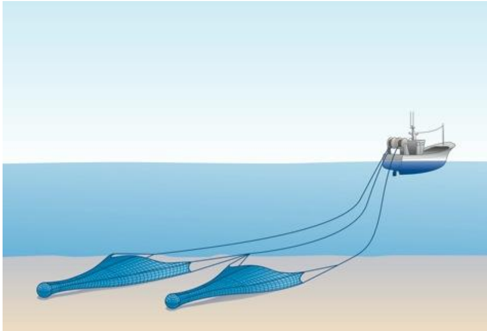
Multi-rig otter trawl
